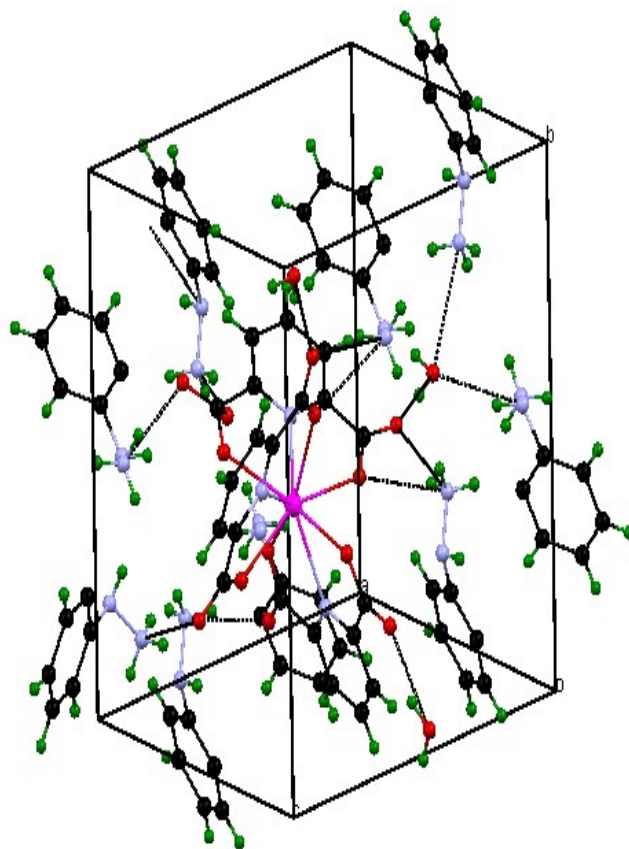
Fig. 2 Packing diagram of lanthanum complex
